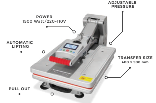
SUBLIMATION PRESS MACHINE
