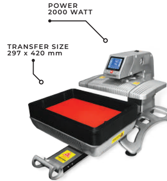
3D SUBLIMATION PRESS MACHINE
