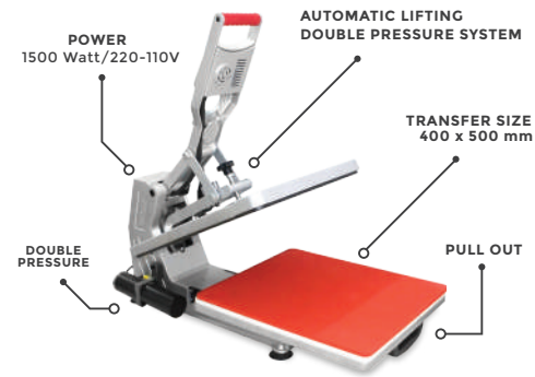
SUBLIMATION PRESS MACHINE DOUBLE PRESSURE
